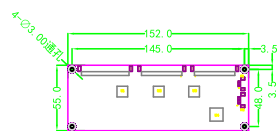
SCALE (3:1) ILITEK 2325 Controller
